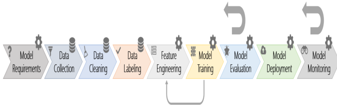
Fig.1.1 Detailed steps for model monitoring
